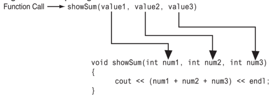
Figure 6-7 Multiple arguments
