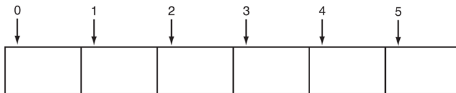
Figure 7-4 Subscripts Subscripts
