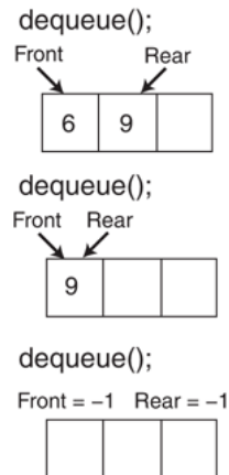
Figure 19-10 State of the queue
