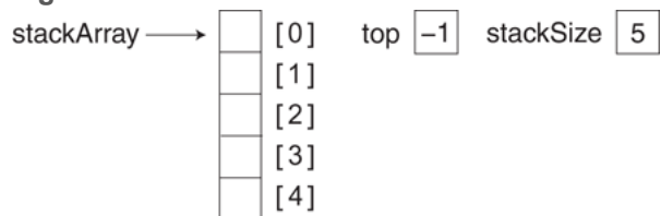
Figure 19-4 State of the stack
