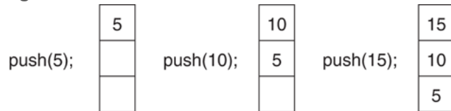
Figure 19-2 State of the stack
