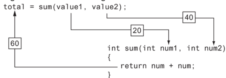
Figure 6-11 A function's arguments and return value
