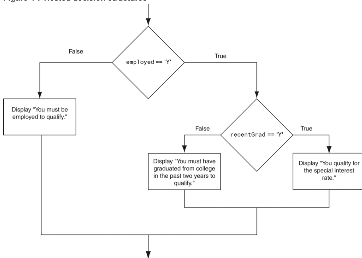
Figure 4-7 Nested decision structures
