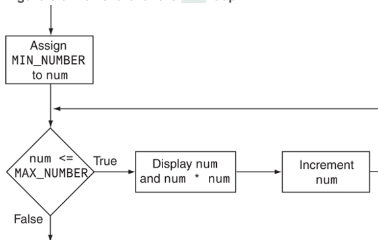
Figure 5-9 Flowchart for the for loop
