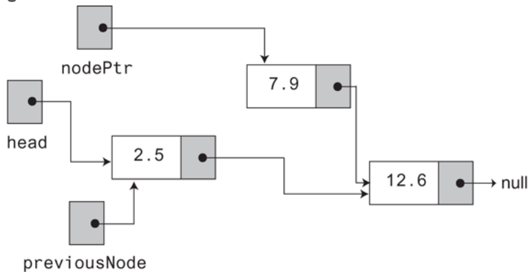
Figure 18-17 Node removed from the list
