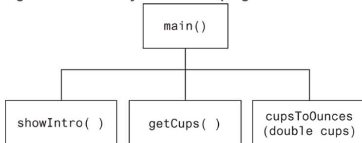
Figure 6-13 Hierarchy chart for the program
