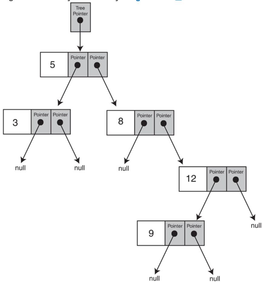
Figure 21-5 Binary tree built by Program 21-1
