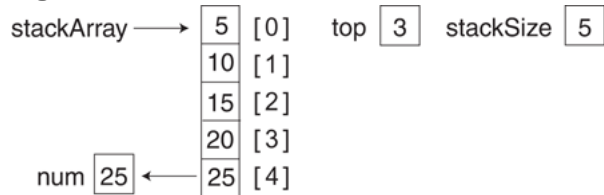
Figure 19-7 State of the stack
