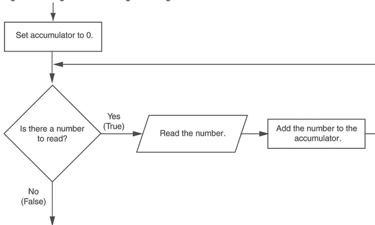
Figure 5-11 Logic for calculating a running total
