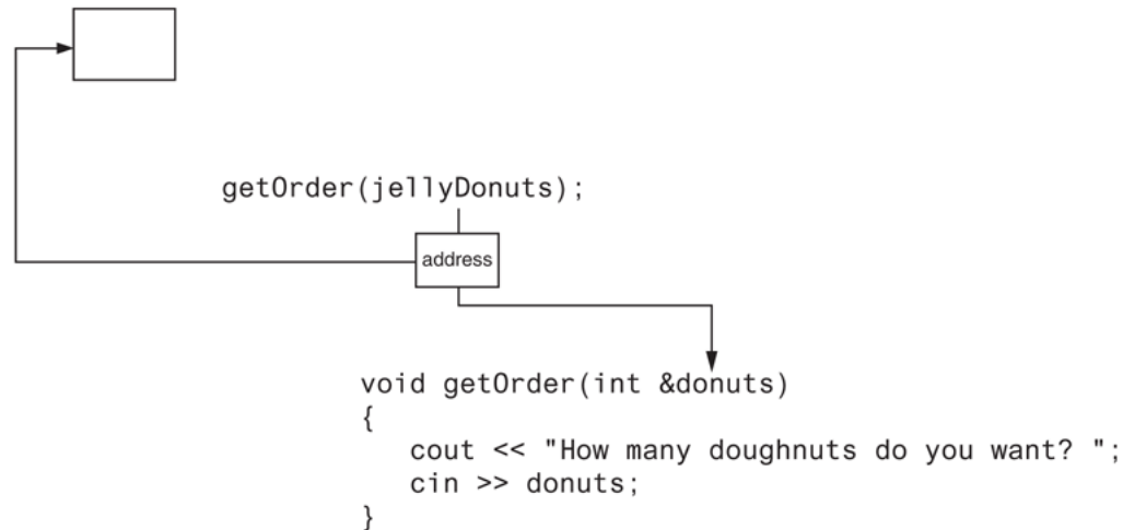
Figure 9-3 Passing an argument by reference jellyDonuts variable
