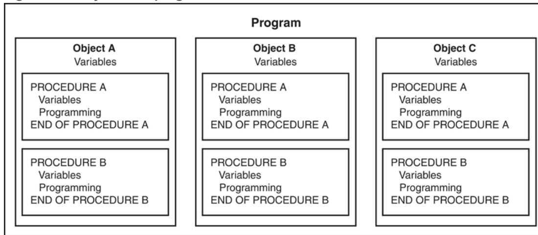
Figure 1-14 Objects in a program
