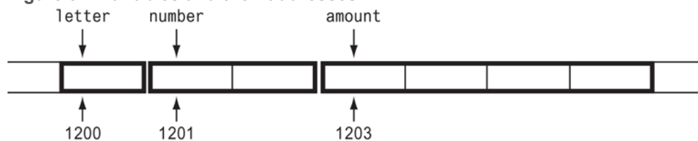
Figure 9-1 Variables and their addresses
