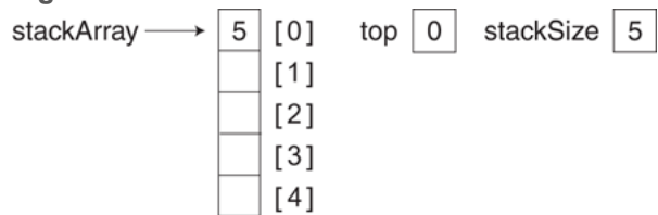
Figure 19-5 State of the stack
