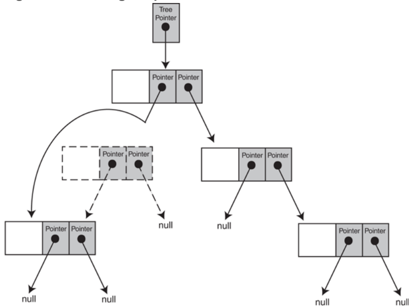
Figure 21-7 Linking the parent node with the subtree
