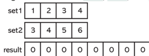
Figure 17-6 State of set1 , set2 , and result after line 15 has executed
