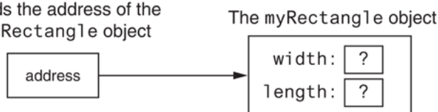
Figure 13-10 rectPtr points to the myRectangle object
