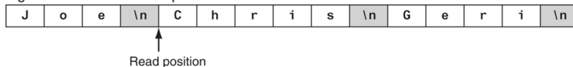
Figure 5-20 The next read position
