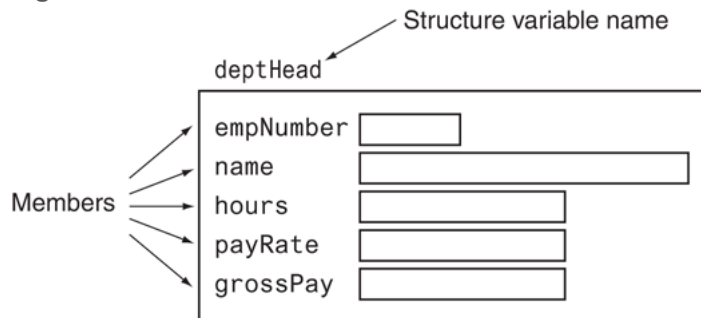
Figure 11-1 A structure and its members
