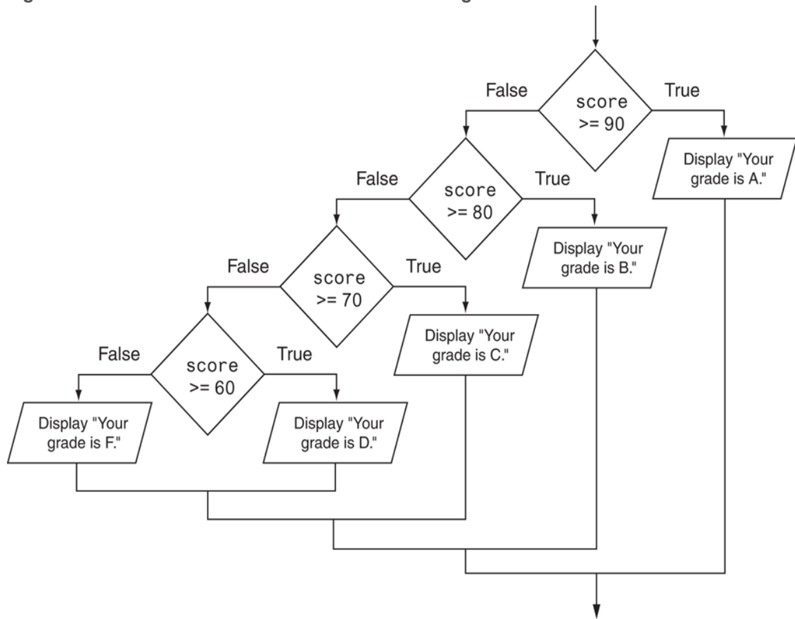
Figure 4-9 Nested decision structure to determine a grade
