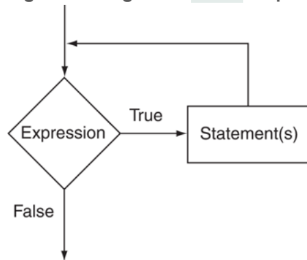
Figure 5-1 Logic of a while loop
