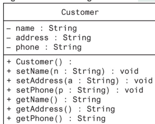
Figure 13-23 UML diagram for the Customer class
