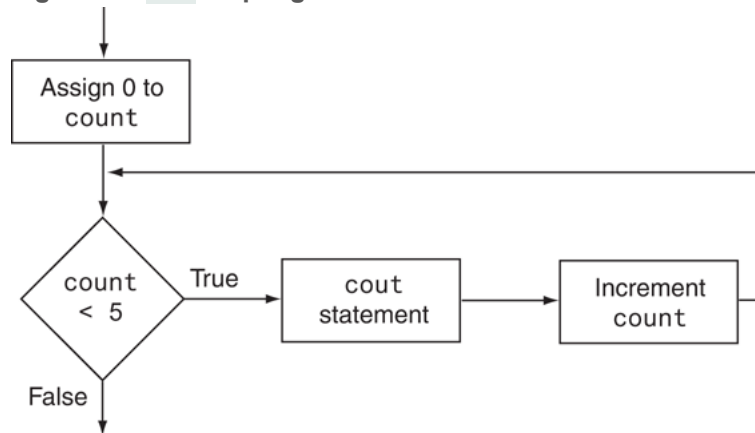
Figure 5-7 for loop logic
