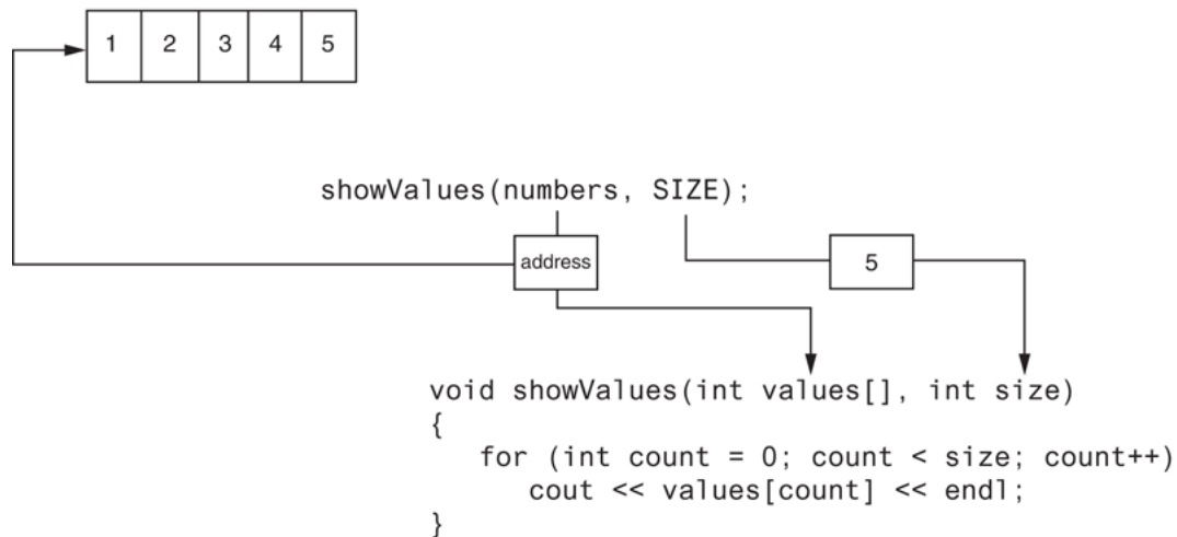
Figure 9-2 Passing an array to a function numbers array
