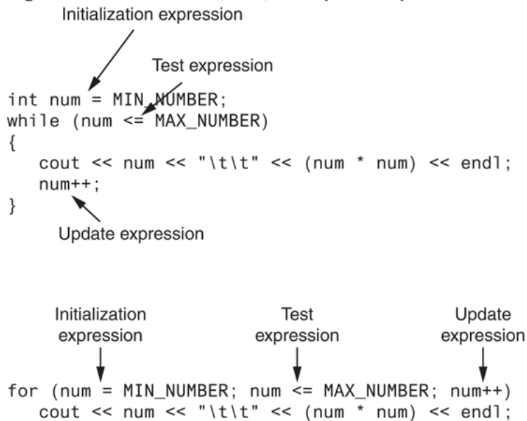
Figure 5-10 Initialization, test, and update expressions
