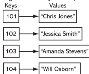
Figure 17-4 Key–value pairs
