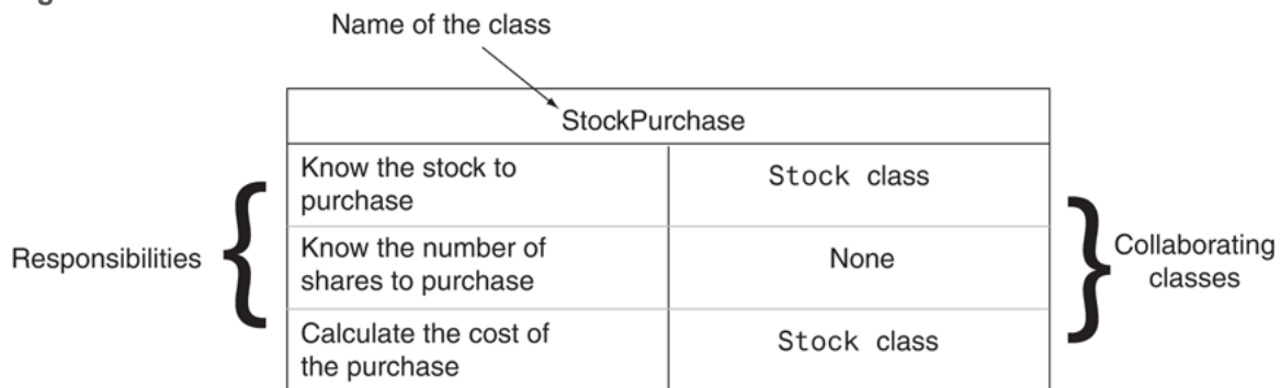
Figure 14-8 CRC card
