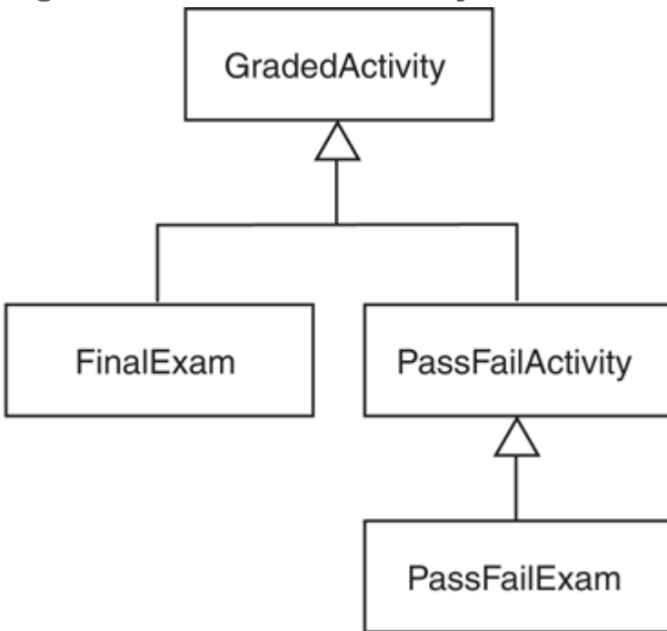
Figure 15-5 Class hierarchy
