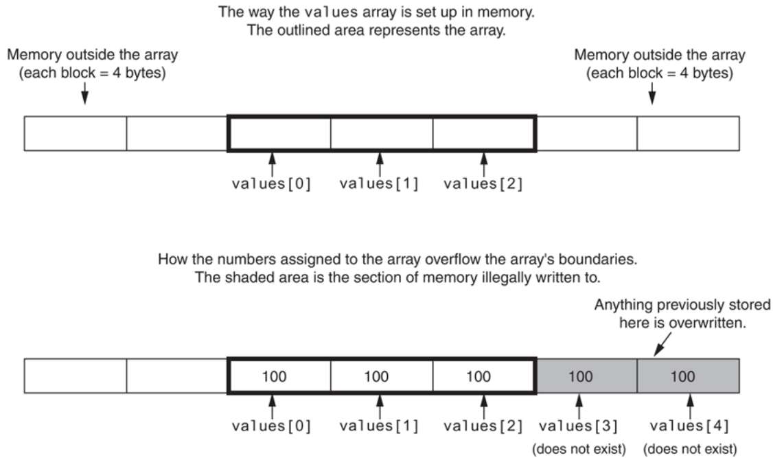
Figure 7-11 Writing data beyond the bounds of an array
