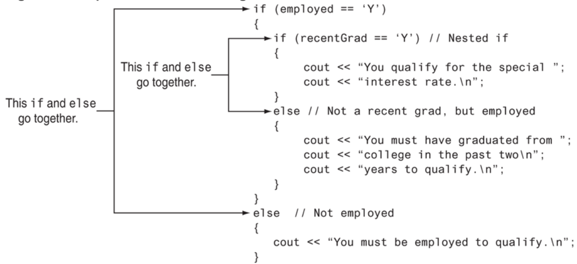
Figure 4-8 Proper indentation and alignment
