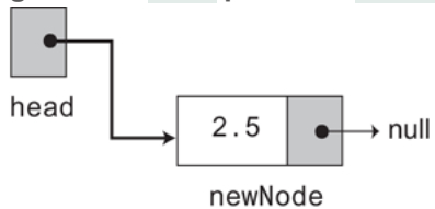
Figure 18-4 head points to newNode
