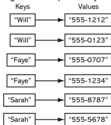
Figure 17-5 Duplicate keys stored in a multimap container
