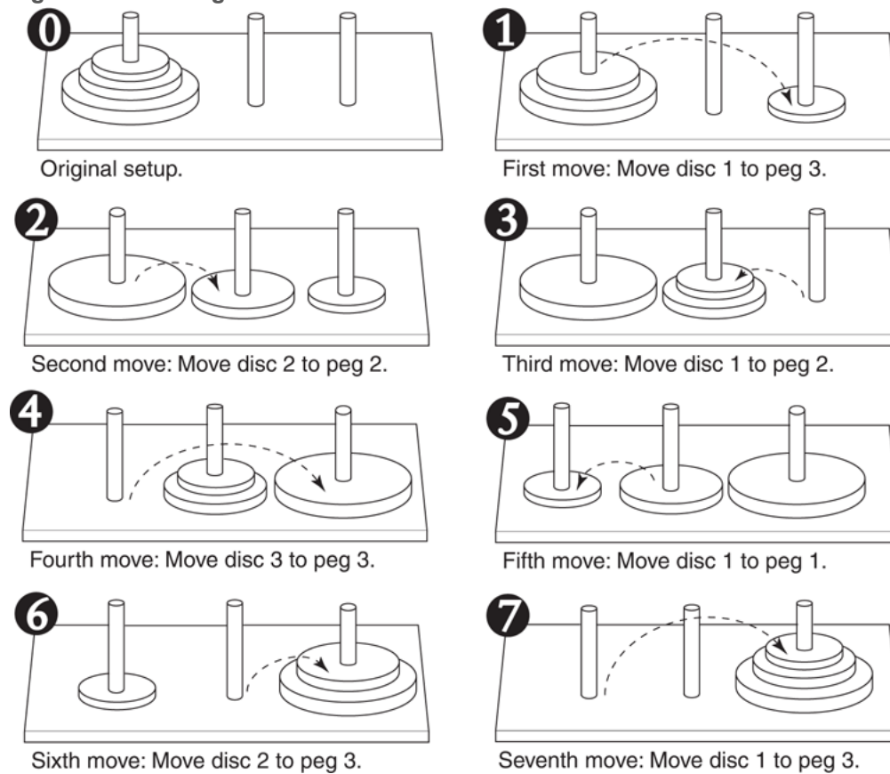
Figure 20-5 Moving three discs
