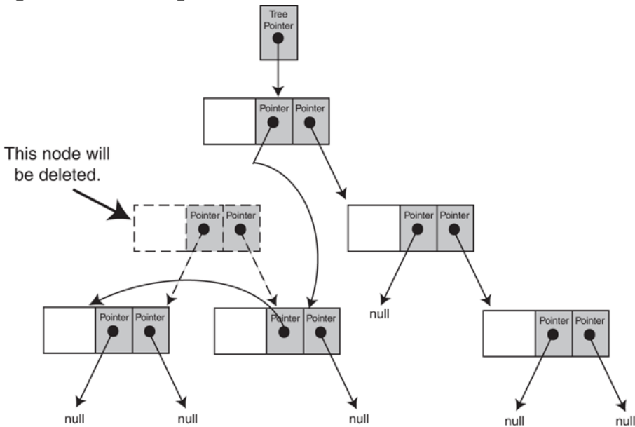
Figure 21-9 Relinking the subtrees
