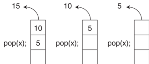
Figure 19-3 State of the stack
