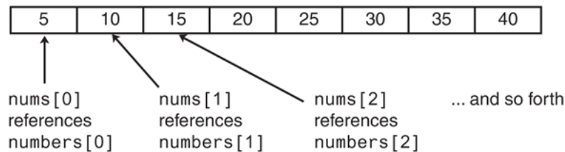
Figure 7-14 Relationship between the numbers array and the nums parameter numbers Array of eight integers
