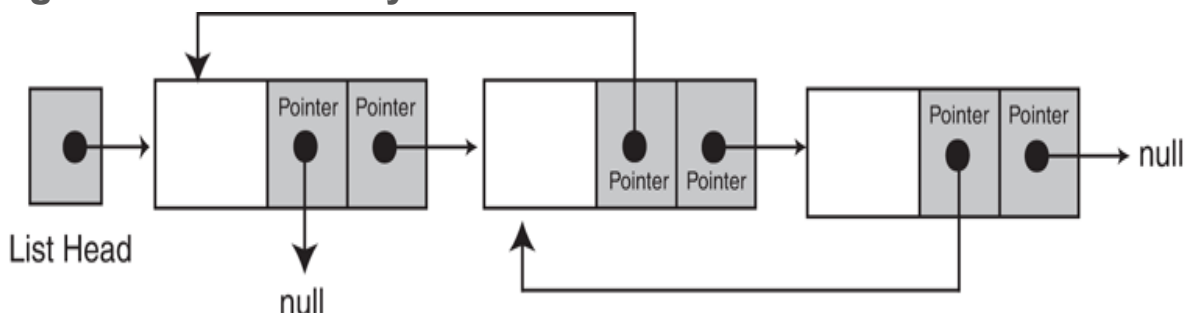
Figure 18-18 A doubly linked list
