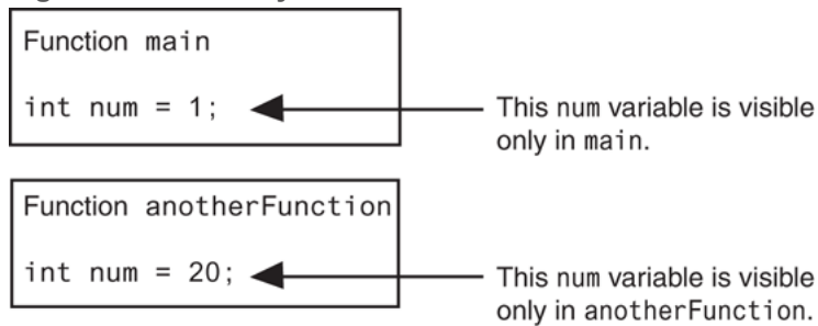
Figure 6-14 Visibility of local variables
