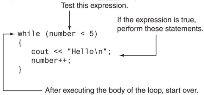
Figure 5-2 Actions of the while loop
