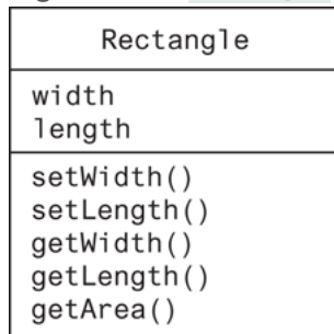
Figure 13-19 Rectangle class
