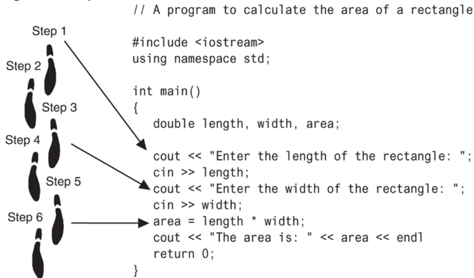
Figure 4-1 Sequence structure
