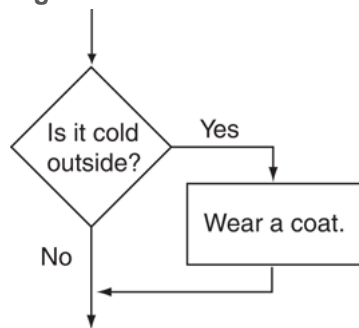
Figure 4-2 Decision structure
