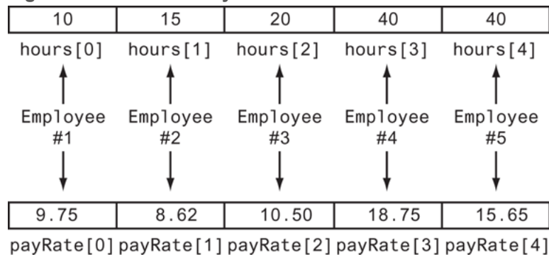
Figure 7-13 Parallel arrays
