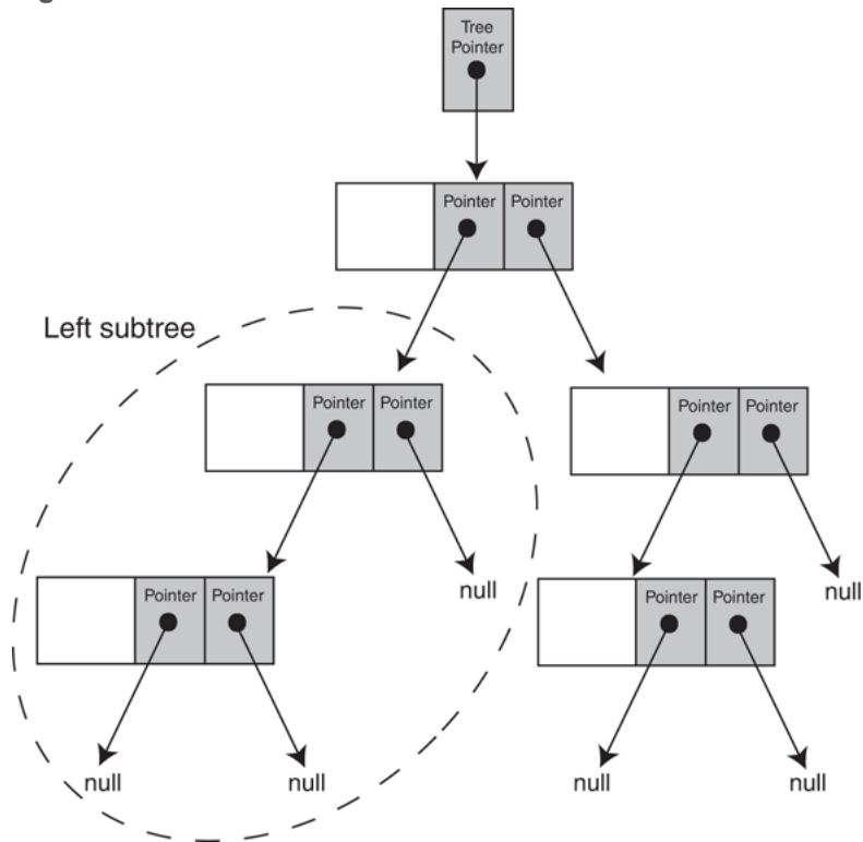
Figure 21-2 Left subtree
