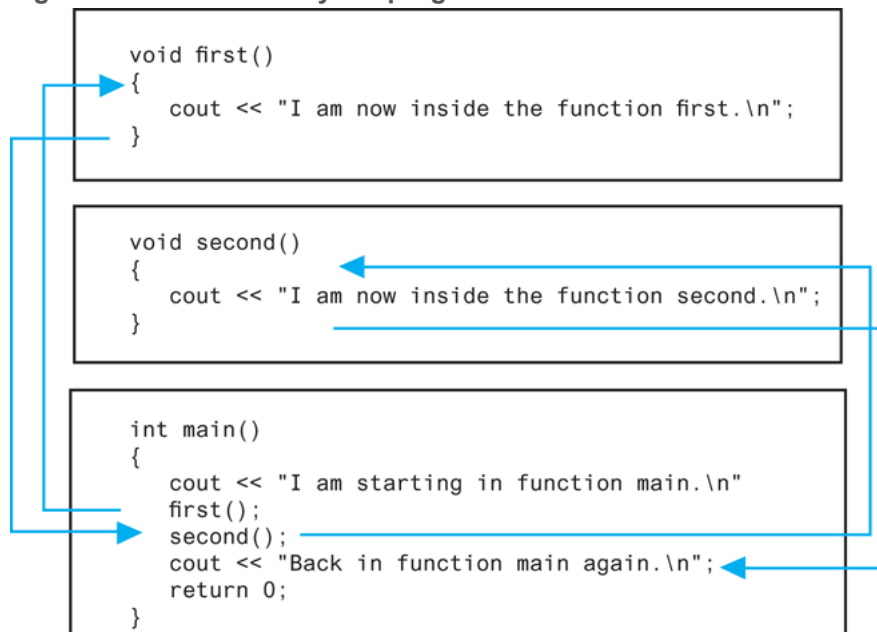
Figure 6-4 Paths taken by the program
