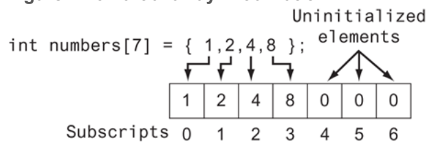
Figure 7-10 Partial array initialization
