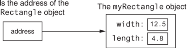
Figure 13-11 State of the myRectangle object
