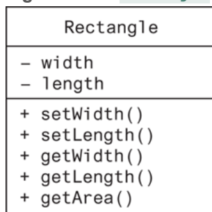
Figure 13-20 Rectangle class with access specification
