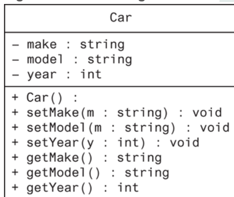
Figure 13-24 UML diagram for the Car class
