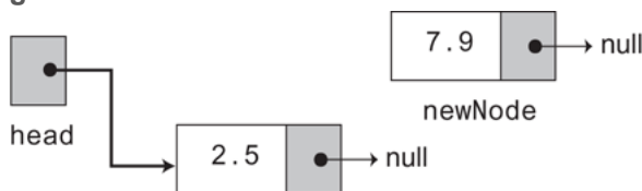
Figure 18-5 A new node is created
