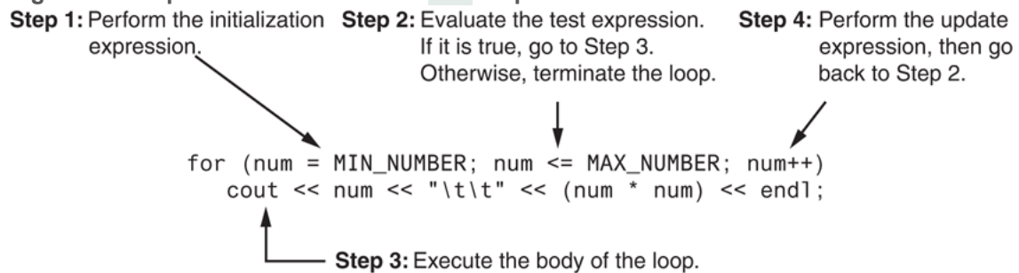
Figure 5-8 Sequence of events in the for loop
