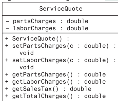
Figure 13-25 UML diagram for the ServiceQuote class
