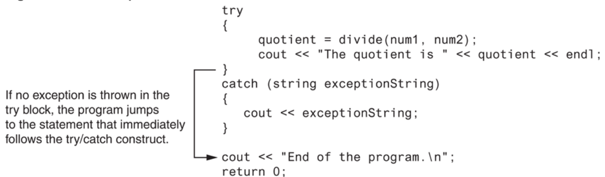
Figure 16-2 No exception was thrown
