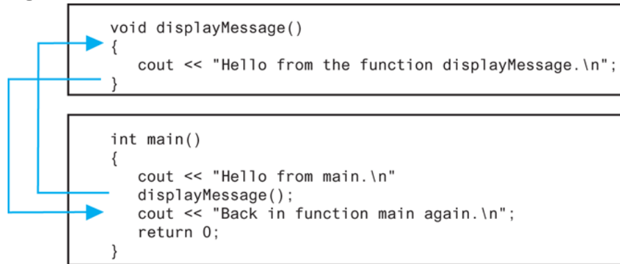
Figure 6-3 A function call
