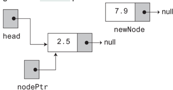
Figure 18-6 nodePtr points to the first node
