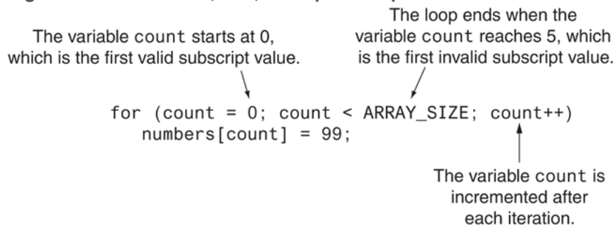
Figure 7-8 Initialization, test, and update expressions
