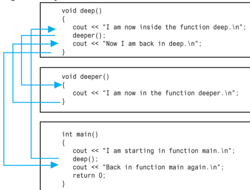
Figure 6-5 Layered function calls
