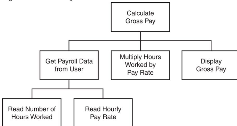
Figure 1-12 Hierarchy chart
