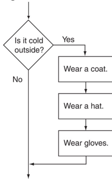
Figure 4-3 Decision structure
