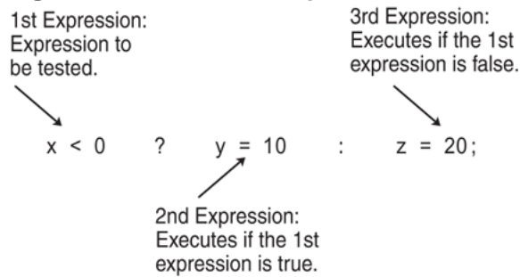
Figure 4-10 Conditional expression
